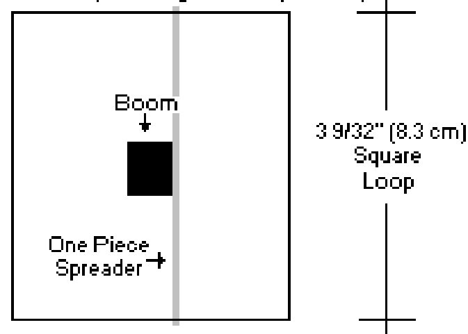
Reflector (total length 13 1/8" (33.4 cm))
