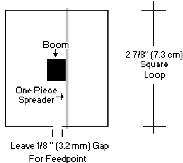
Driven Element (total length 11 3/8" (28.9 cm))
